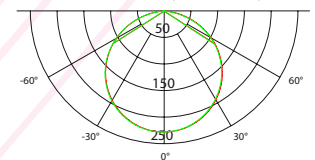
PHOTOMETRIC OF 1M LUMINAIRE (D6300H-24V-8mm)
