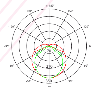
PHOTOMETRIC OF 1M LUMINAIRE (D6280H-24V-10mm)
