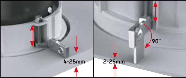
ceiling thickness 4mm to 25mm
